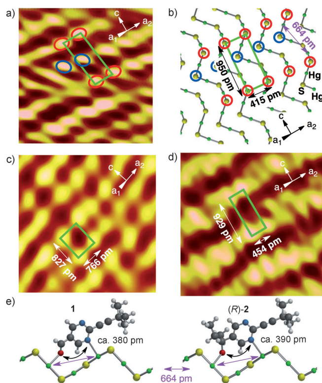
Figure 2. a) AFM images of the (10–10) surface of bare ( P )-HgS (3.5 nm sq.). b) Model of the (10–10) surface of ( P )-HgS. c) Aldehyde 1 adsorbed at the ( P )-HgS (5.0 nm sq.). d) ( R )- 2 adsorbed at ( P )-HgS (3.4 nm sq.). e) Proposed adsorption geometries of 1 and ( R )- 2 at ( P )-HgS. S atoms of the highest level (red circles), S atoms of the second-highest level (blue circles), surface unit cell (green rectangles).
